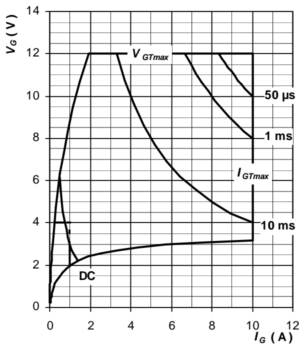
Fig. 5 Maximum peak gate power loss
