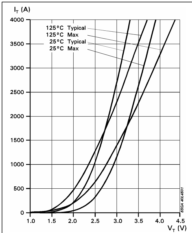
Fig. 2 On-state characteristics
